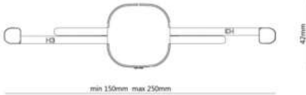
Adjustable two-arm security brackets for tablets OP122-XL
