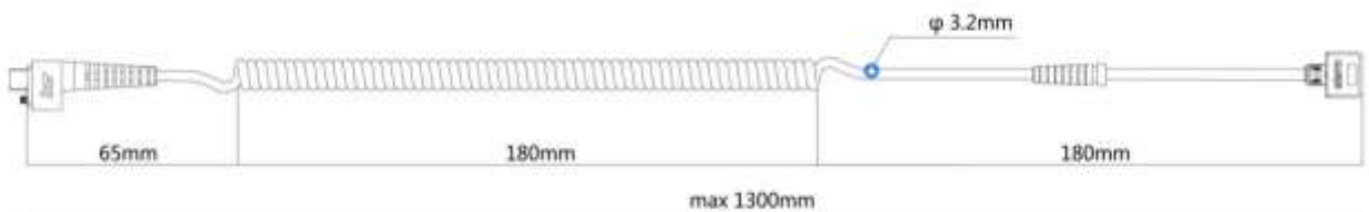
White coiled charging cable with Micro connector(Oposite)
