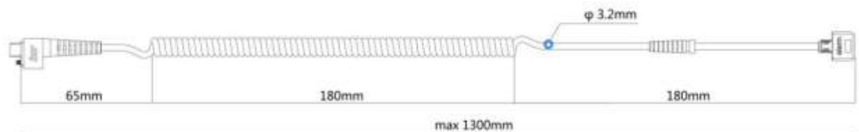
White coiled charging cable with Micro connector
