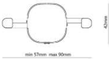
Adjustable two-arm security brackets for phones OP121
